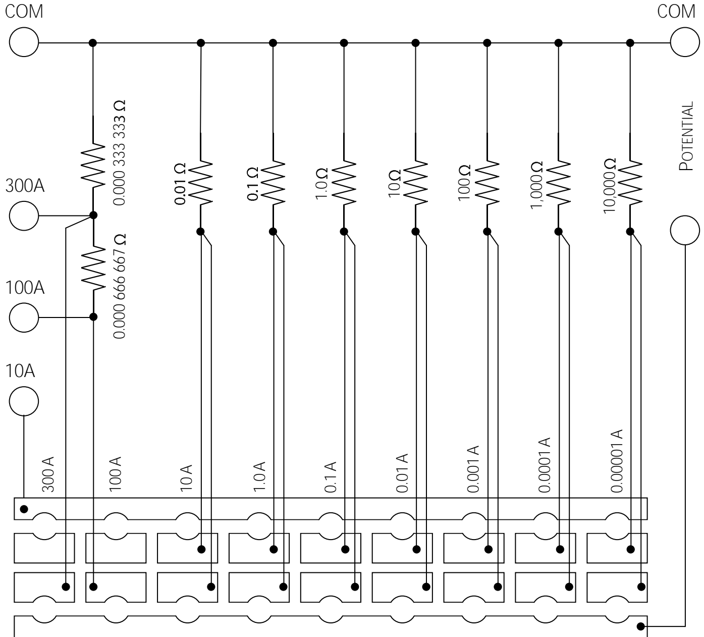
Figure 5-1 : 9711B Schematic Overview
