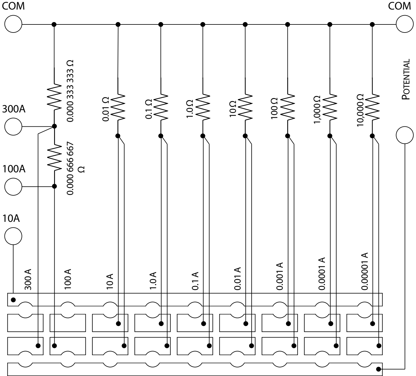
Figure 5-1 : 9711B Schematic Overview
