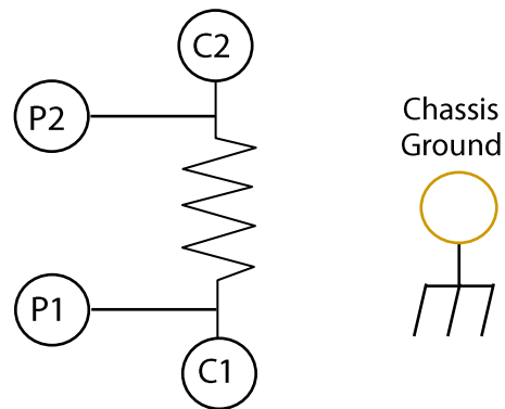
Figure 3-3: 7334 Series from 1 Ω to 10 kΩ
