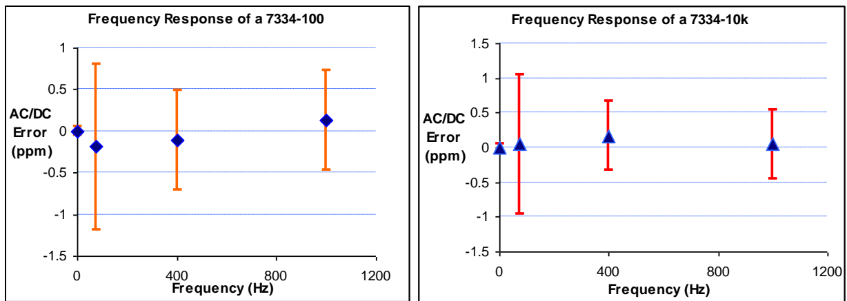
Figure 3-4: AC/DC error of a 7334-100 \Omega and a 7334-10k \Omega Calibrated by UK National Physical Laboratory (NPL)
