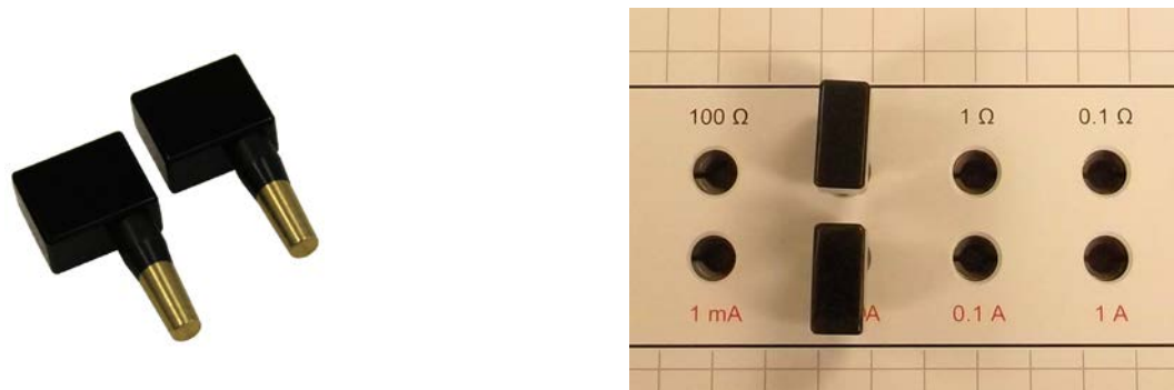
Figure 3-3 : Range Selector Plugs
