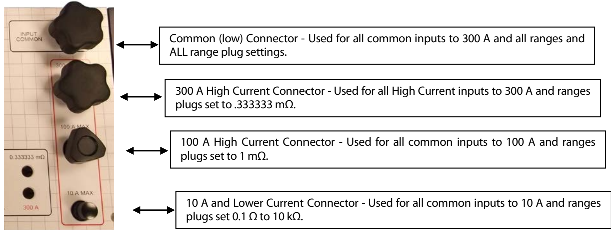
Figure 3-2 : 9211A Current Terminal Connections
