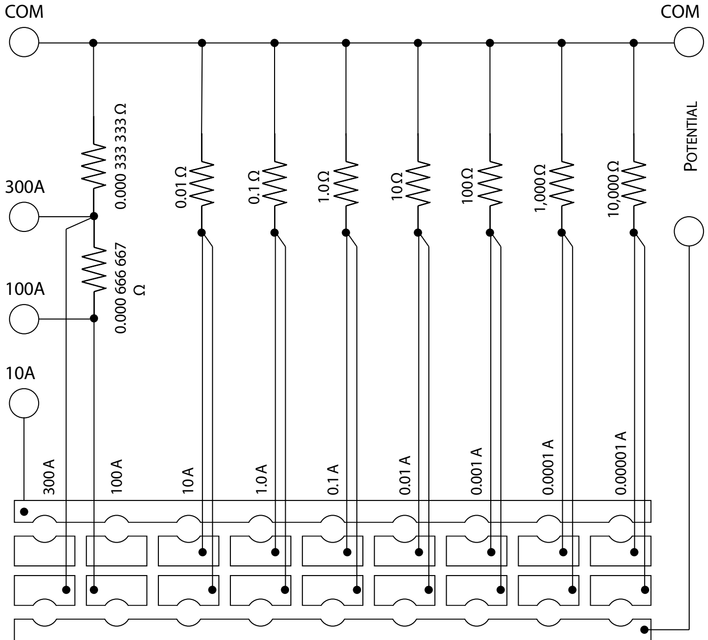
Figure 5-1 : 9211A Schematic Overview
