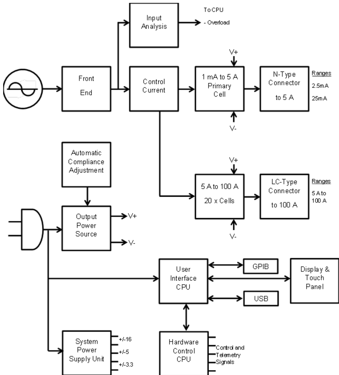
Figure 4-1 : Model 7810 Block Diagram
