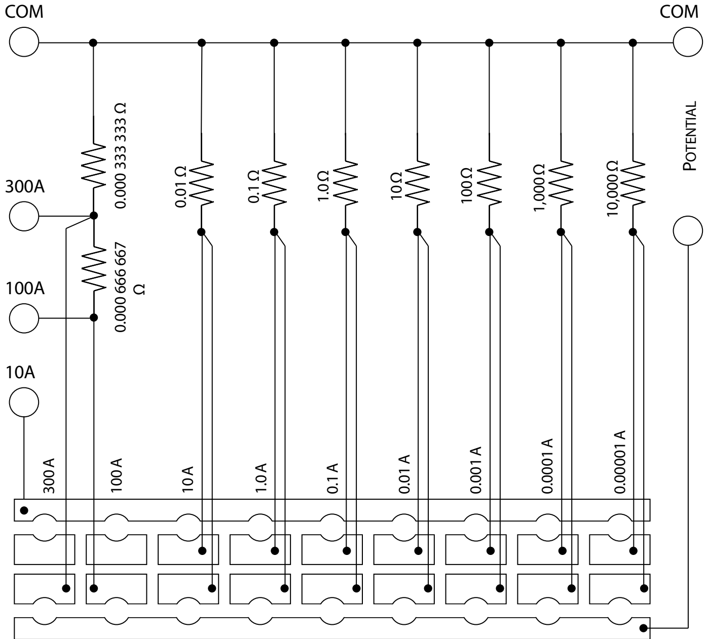
Figure 5-1 : 9211B Schematic Overview
